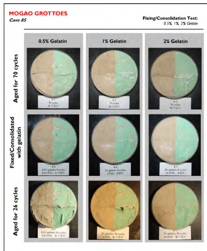
FIGURE 6 Painted plaster disks (loaded with 2% NaCl by wet weight and previously artificially aged for 70 relative humidity cycles [48 hr/100% and 24 hr/ambient RH]) were fixed and consolidated using different amounts of gelatin in water (0.5%, 1%, and 2%). These disks were again cycled to evaluate the performance.
