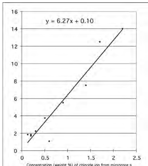
FIGURE 4 Relationship between chloride ion concentration in spot tests and plaster microcores.
