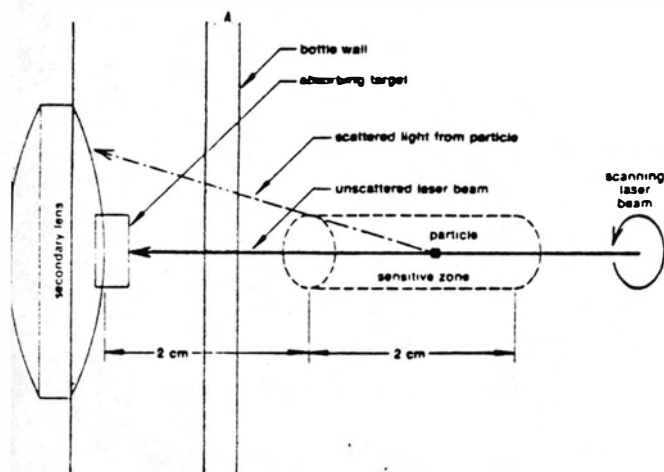
Fig. 2: Laser Beam Optics.
