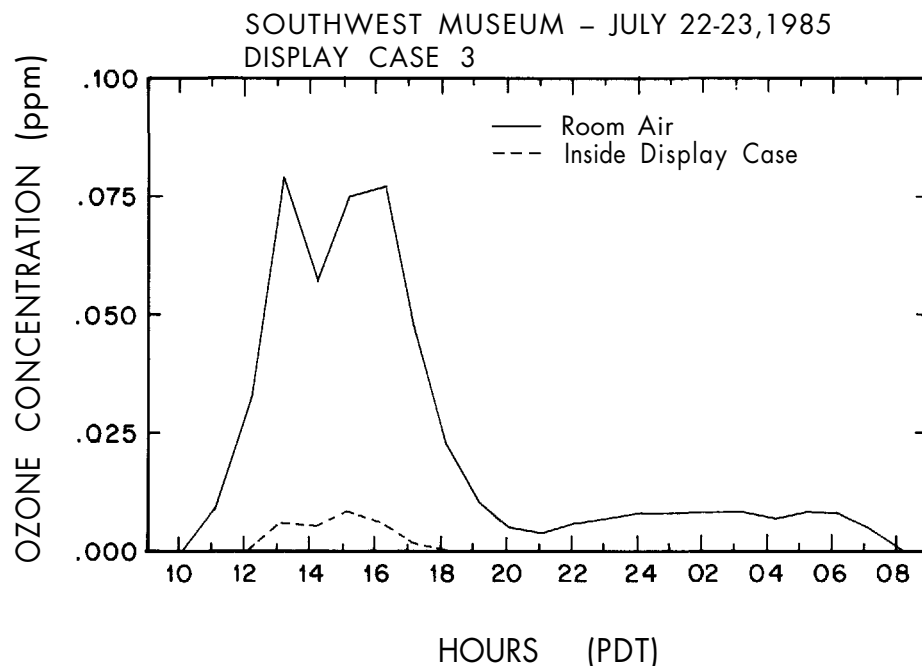
Figure 5.6. Ozone concentrations measured inside Southwest Museum display case 3 and in the surrounding room air, September 22, 1985.
