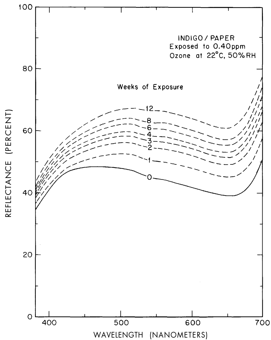
Figure 2.2. Reflectance spectrum of the indigo/paper system at several stages during its exposure to 0.40 ppm ozone at 22 °C, 50% RH, in the absence of light.
