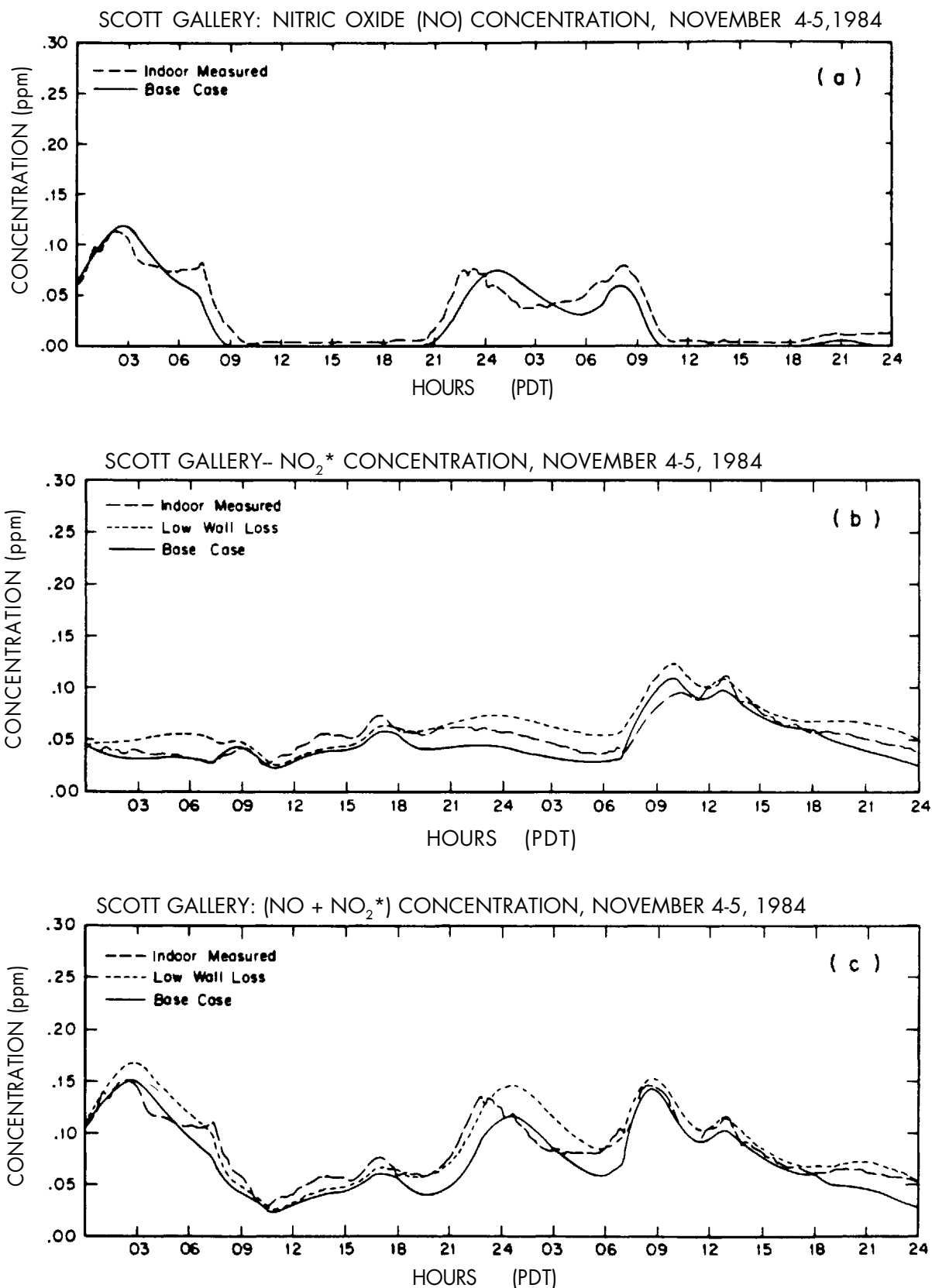
Figure 4.4. Comparison of modeled and measured concentrations of (a) nitric oxide, (b) nitrogen dioxide ( \text{NO}_2^* , measured as \text{NO}_x\text{-NO} ), and (c) total oxides of nitrogen for a two-day period. In the case of nitric oxide, the "base case" and "low ( \text{NO}_2 ) wall loss" simulations produce essentially equivalent results.
