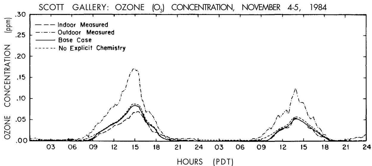
Figure 4.3. Comparison of modeled and measured ozone concentrations for a two-day period.
