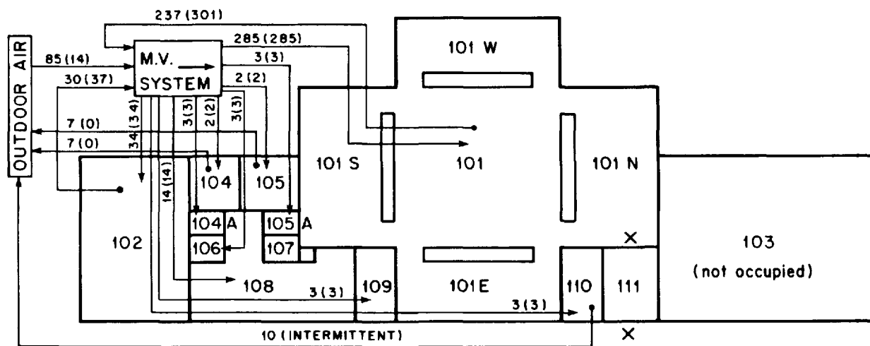
Figure 4.2. Floor plan of the west wing of the Virginia Steele Scott Gallery, San Marino, California. Daytime/(night-time) ventilation flow rates are given in units of \text{m}^3 \text{ min}^{-1} . Air sampling locations for the validation experiment are indicated by "x."
